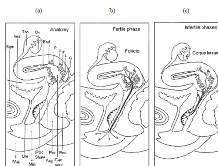
Figure 14. Cervical anatomy and mucus and fluid flow during fertile and infertile phases of the cycle. The locations of crypts P, S, L, and G are indicated as also are F cells (F); I, isthmus (secretion Z); Can cerv, cervical canal; End, endometrium; L. maj., Labium major; L. min., Labium minor; Ov, ovary; Per, perinium; Poo, Shaw, pocket of Shaw; Rec, rectum; Sym, symphysis; Tro, tube; Ure, urethra; Vag, vagina; Ves, bladder.
